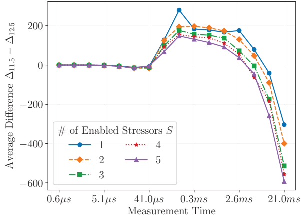
Fig. 10: Difference between the average \Delta metric as measured at 11.5 V and 12.5 V for different measurement times and numbers of stressors enabled on the AC701-1 sink.
