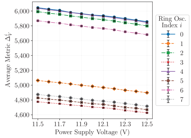
Fig. 9: The average metric \Delta_V^i on the AC701-1 sink decreases with higher power supply voltages V for all eight ring oscillators R_i .
